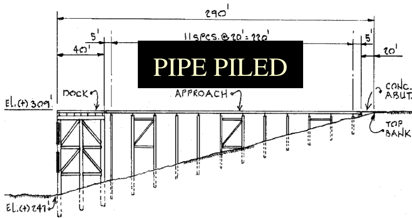
ELEVATION VIEW
