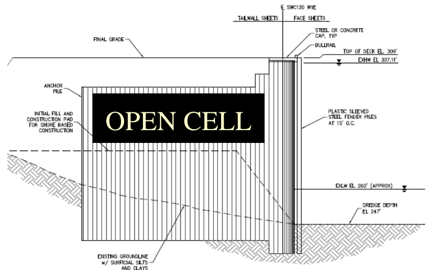
TYPICAL SECTION
